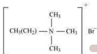
Cetyltrimethylammonium bromide
